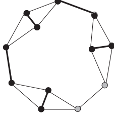
Figure 6: The necklace N_3
